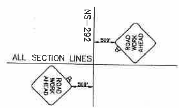
TYPICAL SIGN PLACEMENT SIDE ROADS
