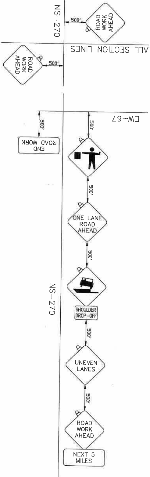
TYPICAL SIGN PLACEMENT SIDE ROADS
