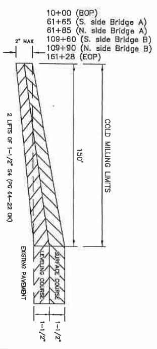
TYPICAL TIE-IN DETAIL
