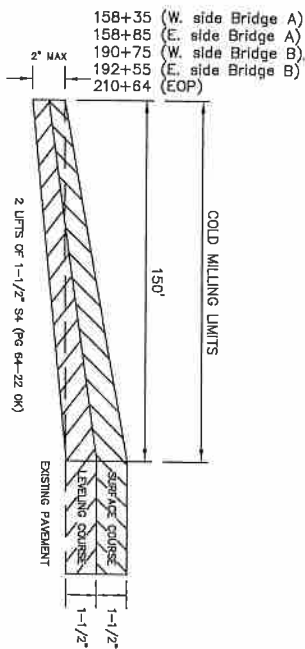
TYPICAL TIE-IN DETAIL
