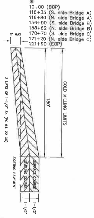
TYPICAL TIE-IN DETAIL
