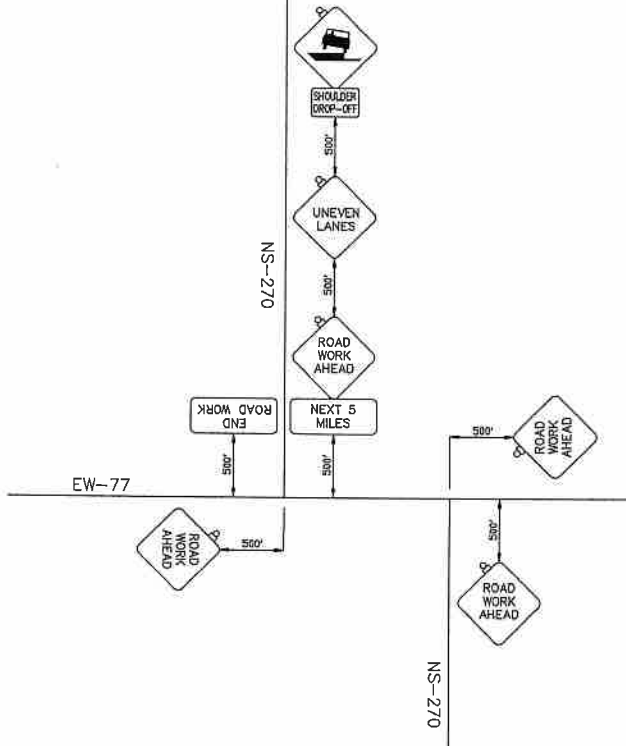
TYPICAL SIGN PLACEMENT NEAR BOP
