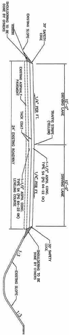
TYPICAL SECTION
